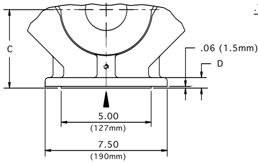
FOR ANSI FLANGE CLASS 150
